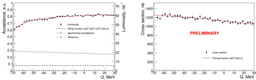
Fig. 3. Left panel: efficiency for pd \rightarrow pd\pi^0 reactions as a function of excess energy Q and integrated luminosity calculated for the experimental data for the quasi-free pd \rightarrow ppn_{spectator} reaction. Right panel: excitation function for pd \rightarrow pd\pi^0 process after applying selection criteria described in the text.
