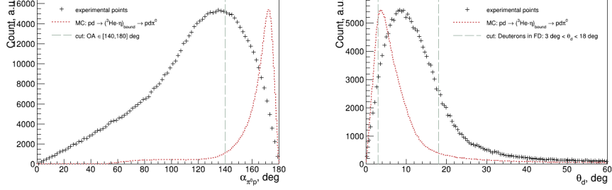
Fig. 2. Left panel: \pi^0 -proton opening angle in the center-of-mass frame \theta_{\pi^0 p}^{cm} . Right panel: Deuteron scattering angle spectrum in the laboratory frame. Vertical dashed lines indicate the applied selection cuts.
