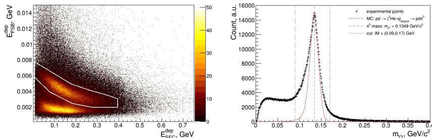
Fig. 1. Left panel: Experimental spectra of the energy loss in the Central Detector. The selected area for protons is marked with white line. Right panel: \pi^0 identification based on invariant mass spectrum of two gamma quanta. Vertical dashed lines indicate the applied selection cut criteria.
